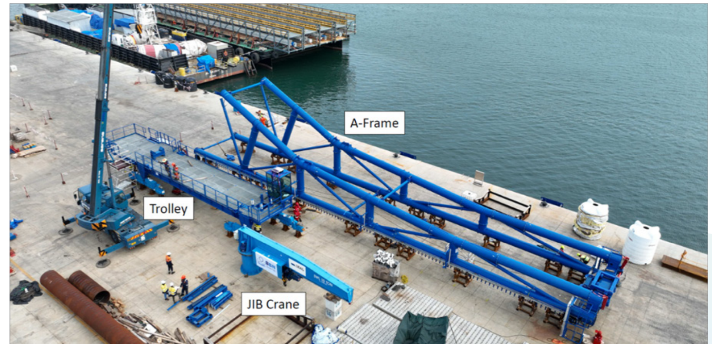
Jetty Assembly of the remaining Launching Girder Elements
