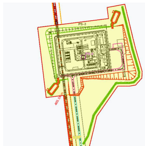
Revised PS3 Footprint Change (2022)
