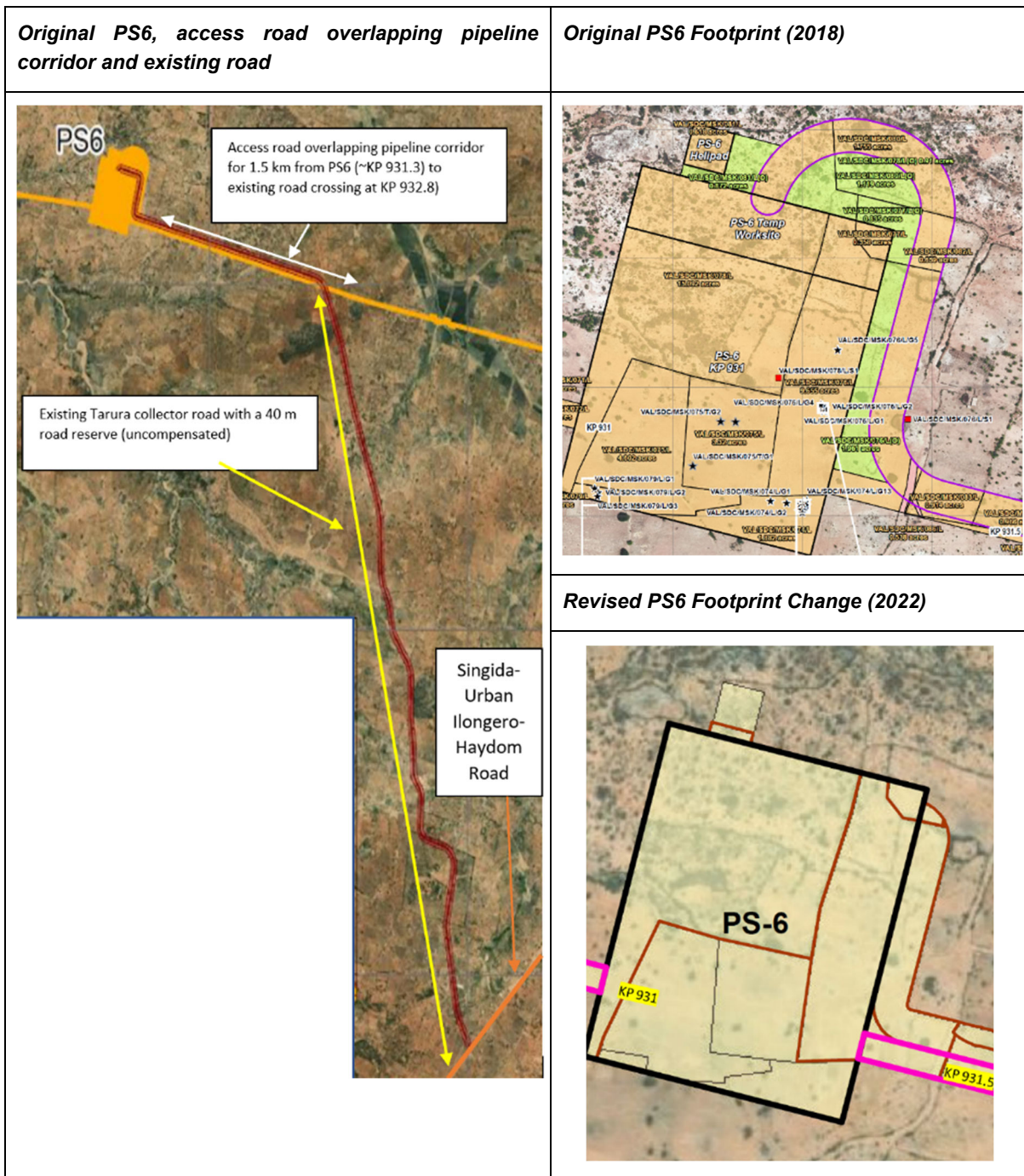
Figure 2-18 Overview of PS6 and Access Arrangements
